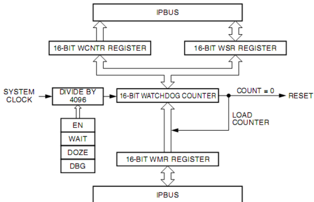
Watchdog Timer Block Diagram
